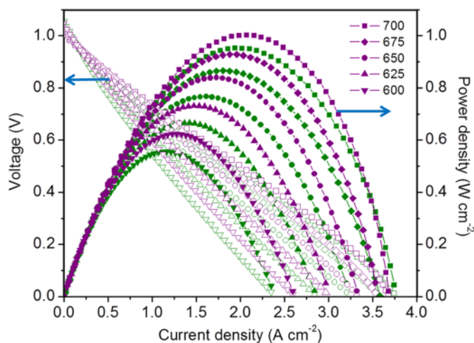
Figure 5 | Stability of the hierarchical LN protected BSCF cathode under working conditions. The cathode was prepared on a YSZ–Ni (50 : 50 vol%) anode supported SDC (5 \mu\text{m} )|YSZ (5 \mu\text{m} ) electrolyte single cell. I–V and I–P curves of the single fuel cell were first tested using air in the cathode side at 600–700 °C (purple curves). After introduction of 10 vol% CO 2 for 1 h, the fuel cell was tested again in CO 2 containing air (green curves).
